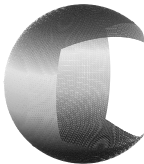
Figure 2-15: Part of a Sphere Formed by Four Rotates of a Quartic Rational
